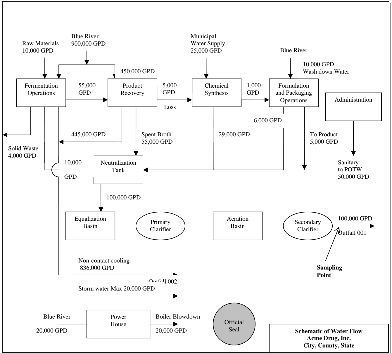
FIGURE 1 - SCHEMATIC FLOW DIAGRAM
