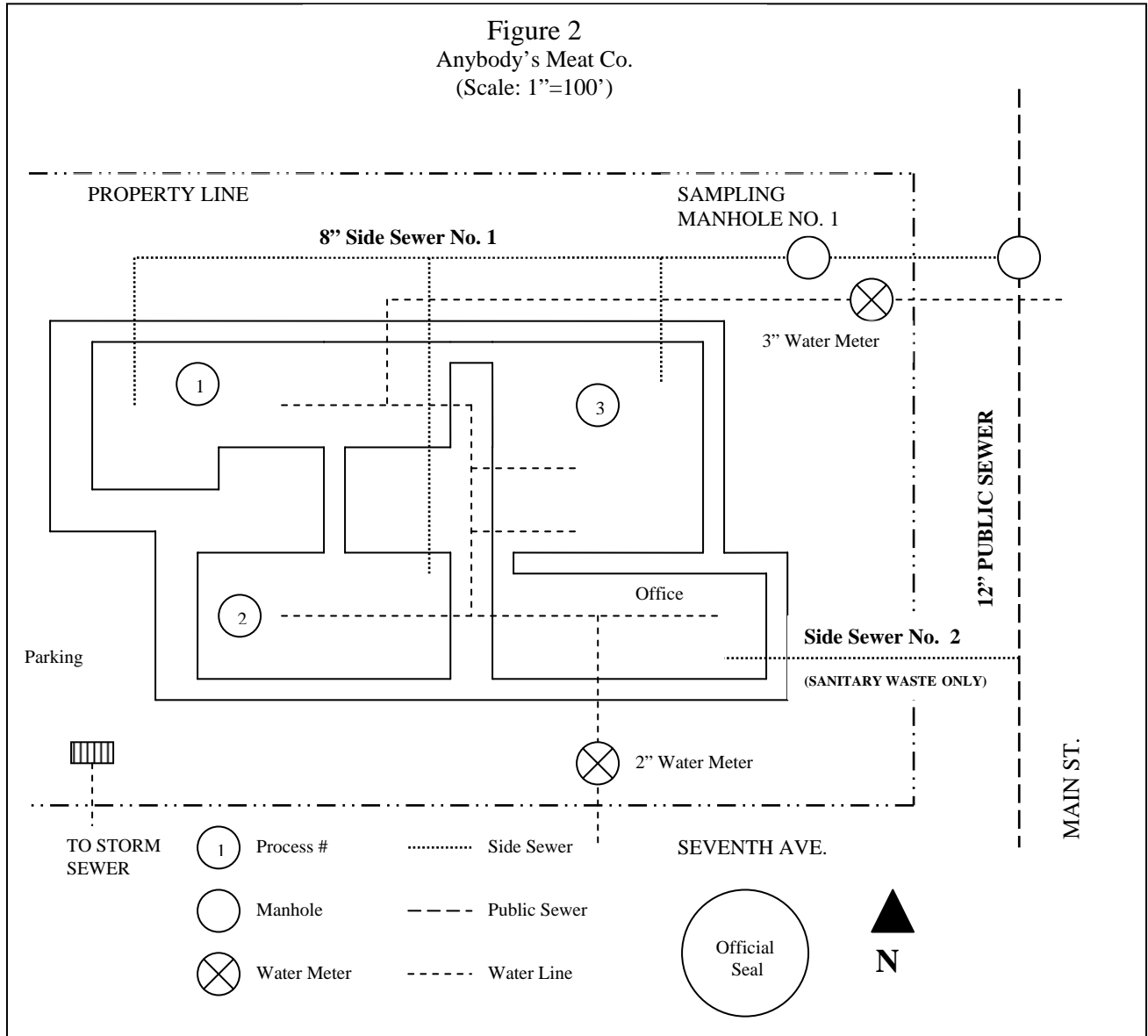
FIGURE 2 - BUILDING LAYOUT
